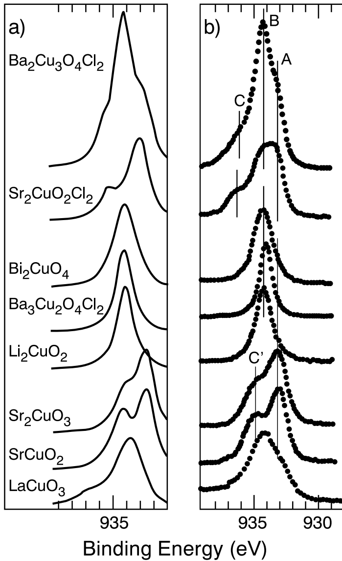
Figure 1: a) Theoretical core level spectra for different divalent and one trivalent \text{LaCuO}_3 cuprate. b) Experimental spectra by Böske et al. for the divalent Cu compounds and by Mizokawa et al. for the trivalent \text{LaCuO}_3 .
